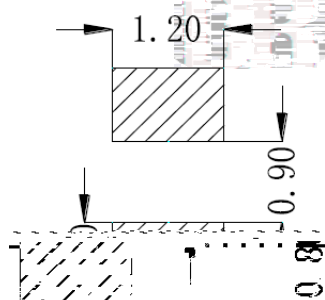
Fig.1-5 Soldering Patterns
