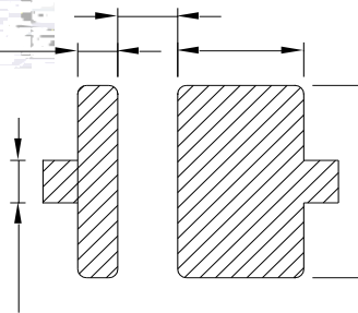
Fig.1-5 Soldering patterns 推荐焊盘
