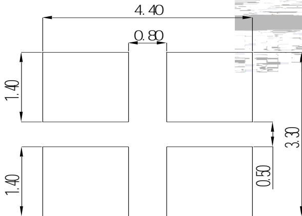
Fig.1-5 Soldering patterns
