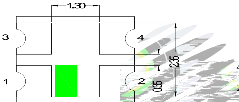
Fig.1-3 Bottom view
