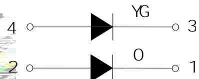
Fig.1-4 Polarity
