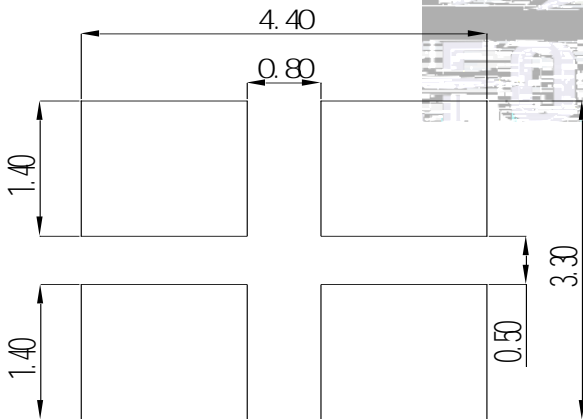
Fig.1-5 Soldering patterns
