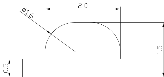
Fig.1-2 Side view
