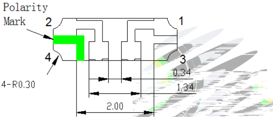
Fig.1-3 Bottom view
