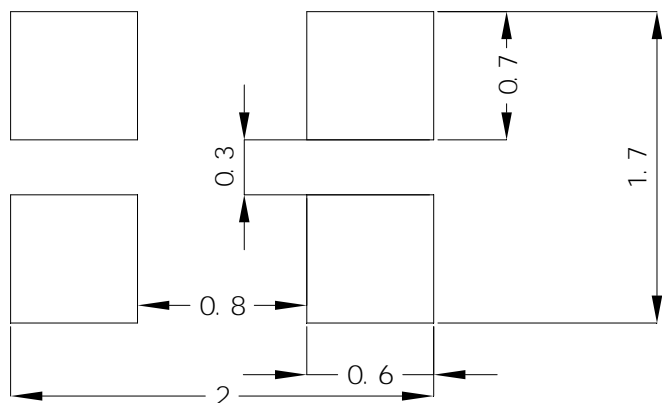
Fig.1-5 Soldering patterns
