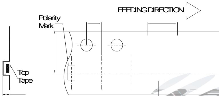
Fig.2-1 Carrier Tape Dimension
