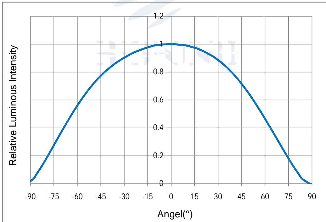
Fig 1-11 Radiation diagram
