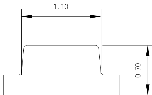
Fig.1-2 Side view
