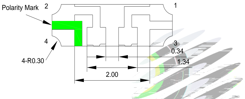
Fig.1-3 Bottom view
