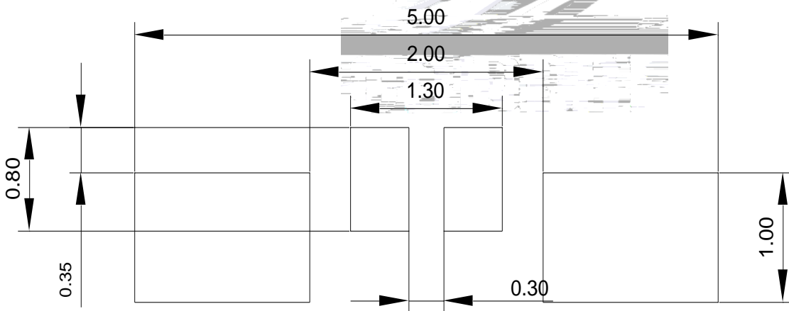
Fig.1-5 Soldering patterns
