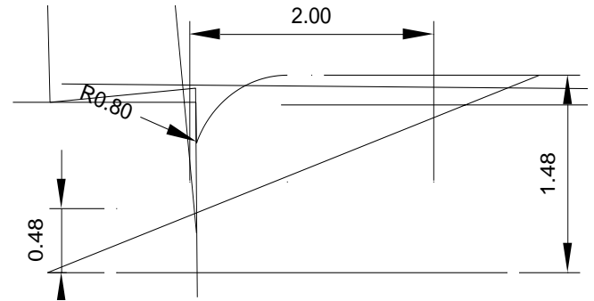
Fig.1-2 Side view
