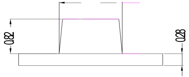
Fig.1-2 Side view
