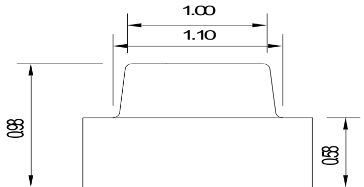
Fig.1-2 Side view
