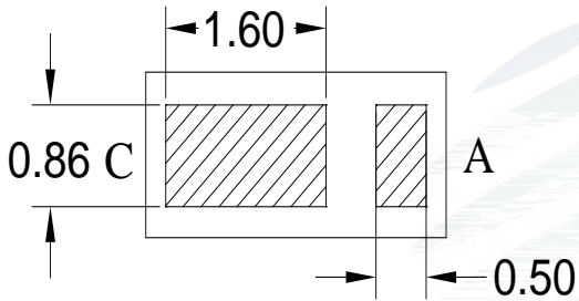
Fig. 1-3 Bottom View
